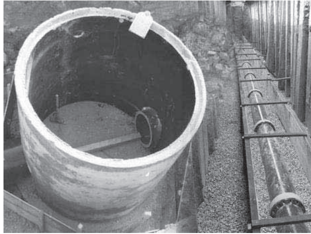
Sewer piping
